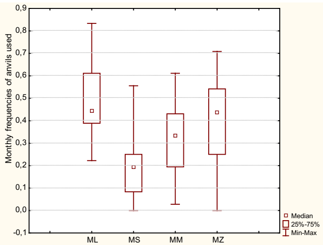
Fig. 6. Box-plots indicating use of anvil sites in the four areas surveyed.
